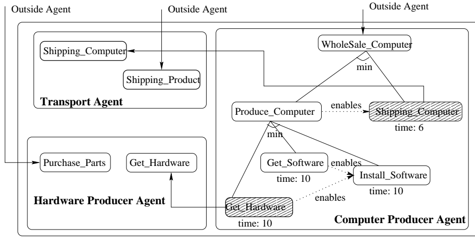
Figure 3: Agent Society
