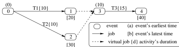
Figure 9: MQ level partial order schedule
