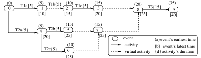
Figure 10: partial order schedule with one non-local subtask
