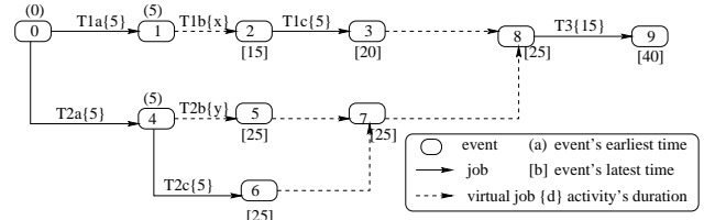
Figure 11: partial order schedule with two indirectly related issues
